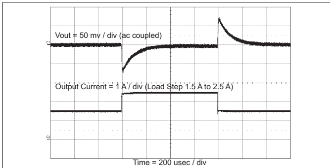
Figure 47. Load Transient
