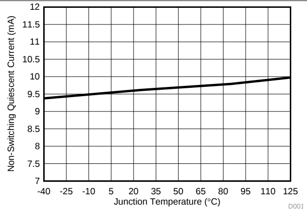
Figure 8. Non-Switching Input Current ( I_{VDD} ) vs. Junction Temperature
