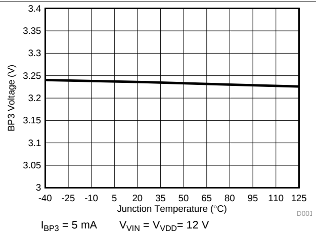
Figure 10. BP3 Voltage vs. Junction Temperature
