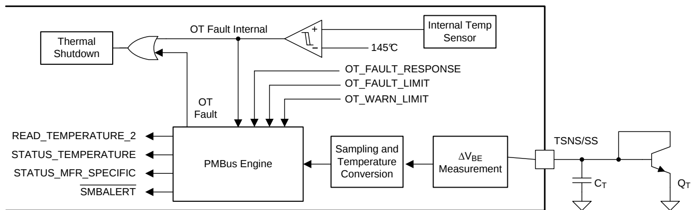
Figure 38. Over-Temperature Protection
