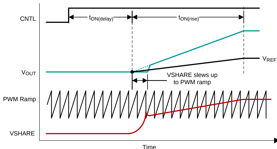
Figure 31. Soft-Start Timing
