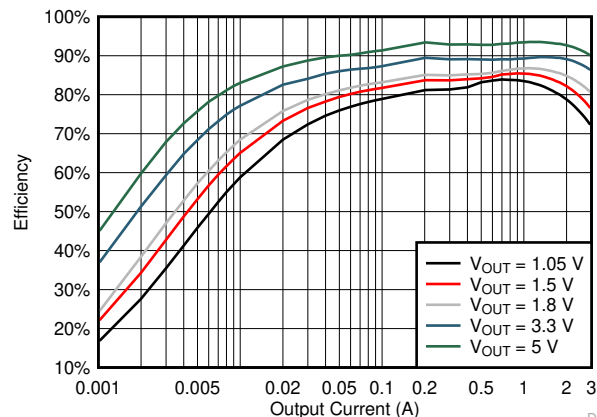
TPS563201 Efficiency
