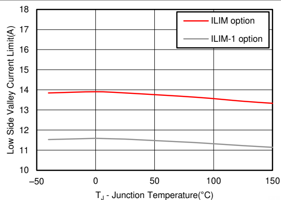
Figure 6-10. Current Limit vs Temperature
