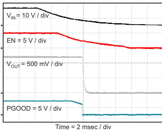
Figure 8-16. Shut Down Relative to V_{IN} Falling
