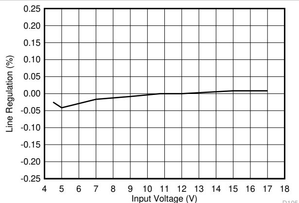
Figure 8-6. Line Regulation, I_{OUT} = 6\text{ A}
