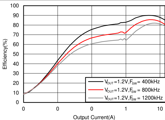
Figure 6-11. Efficiency with Internal VREG5 = 4.7 V, V_{IN} = 12\text{ V}
