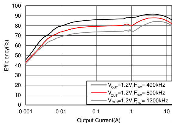
Figure 6-12. Efficiency with External VREG5 = 5 V, V_{IN} = 12\text{ V}
