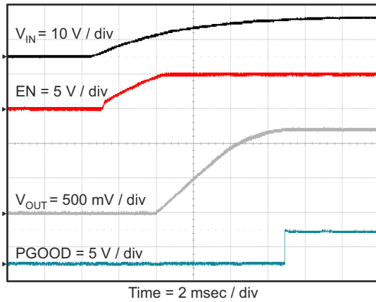
Figure 8-14. Start Up Relative to V_{IN} Rising
