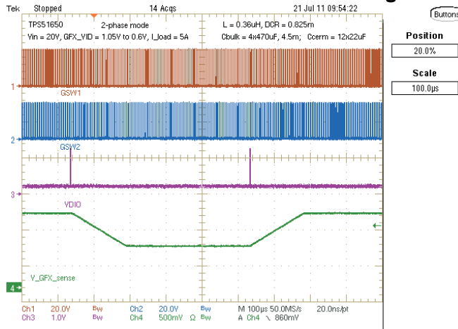
Figure 31. Dynamic VID: V_{IN} = 20\text{ V} , SetVIDSlow = 0.6 V, SetVIDFast = 1.05 V
