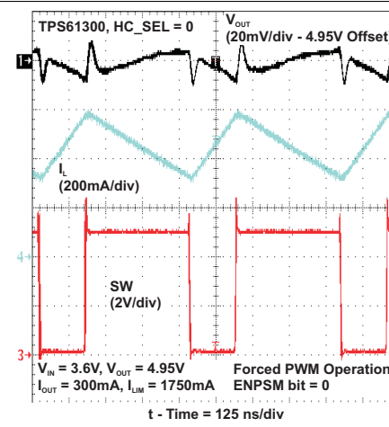
Figure 93. PWM Operation
