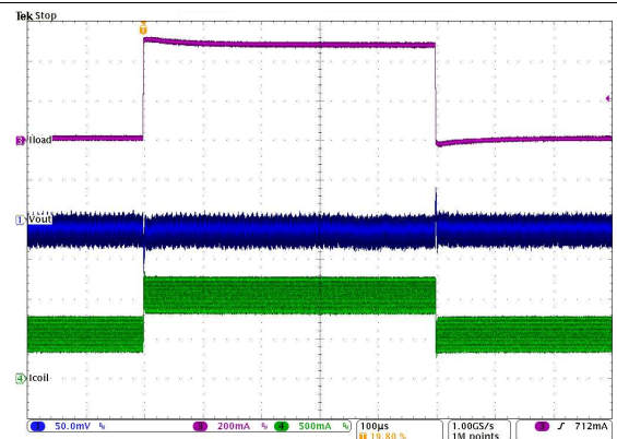
Figure 35. Load Transient Response (0.5 to 1 to 0.5 A)
