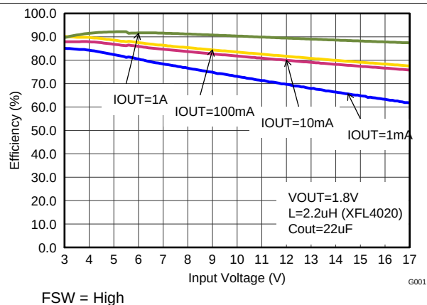
Figure 19. Efficiency vs. Input Voltage
