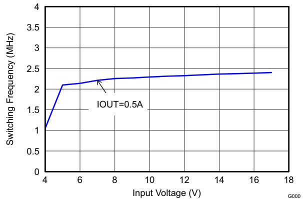
Figure 17. Switching Frequency versus Input Voltage
