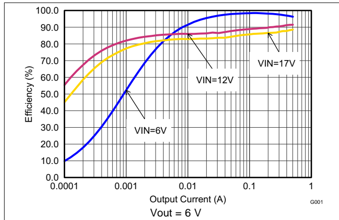
Figure 6. Efficiency versus Output Current
