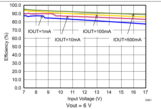
Figure 7. Efficiency versus Input Voltage
