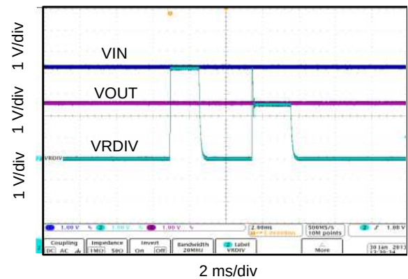
Figure 64. Steady State Operation
