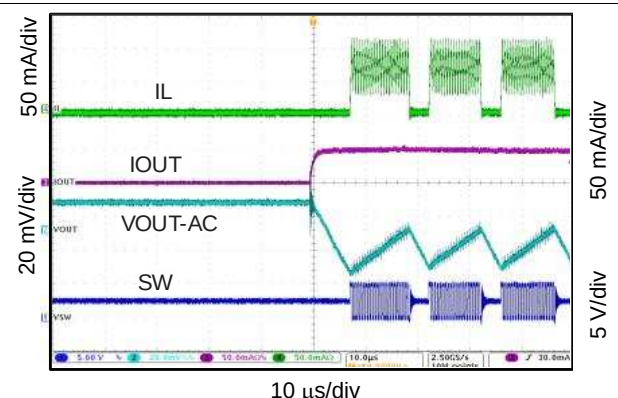
Figure 66. Sampling Waveform
