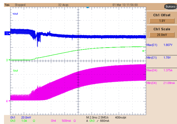
Ch1 = V_{OUT} Ch3 = I_{OUT} Ch4 = Inductor Figure 8-34. Buck 2 PFM to PWM Transition
