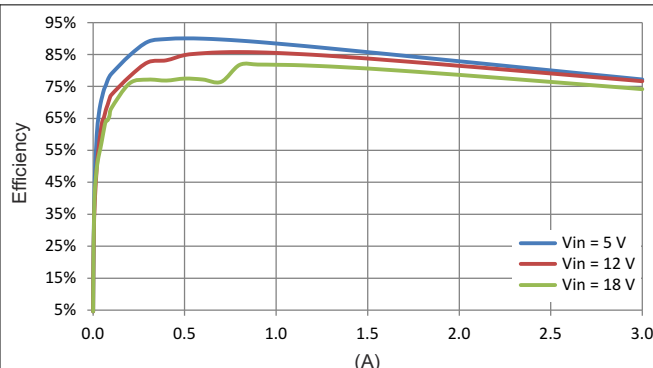
Figure 6-2. Efficiency, LOW_P Mode
