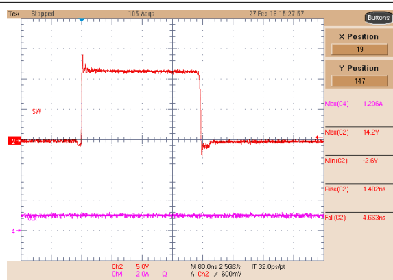
Figure 8-26. Buck 2 Switching Node, 1-A Load
