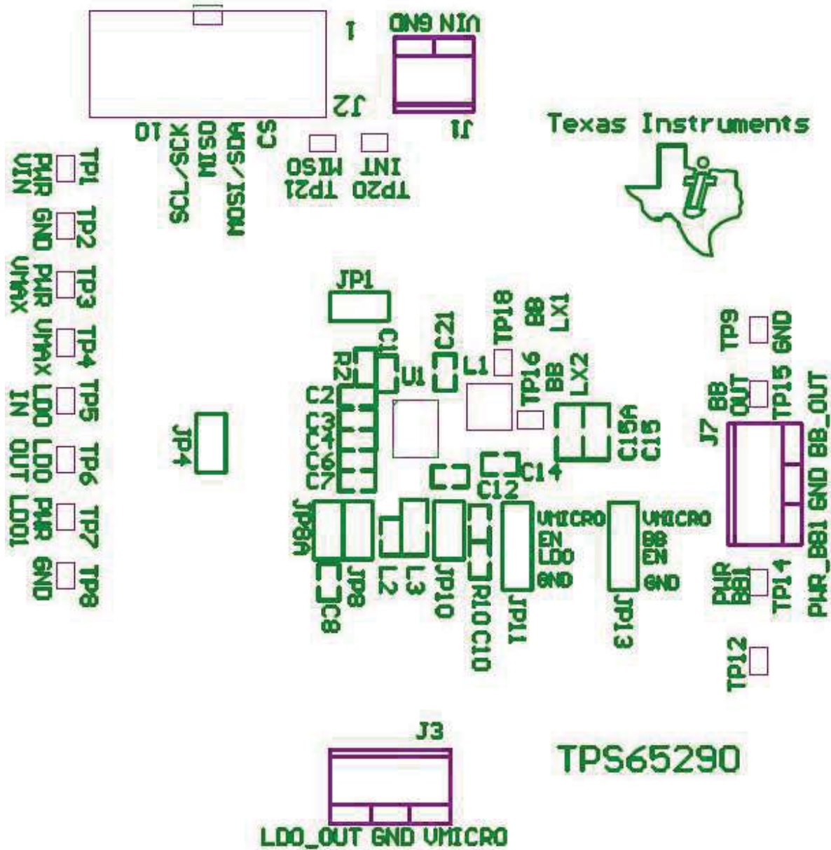
Figure 71. Component Placement
