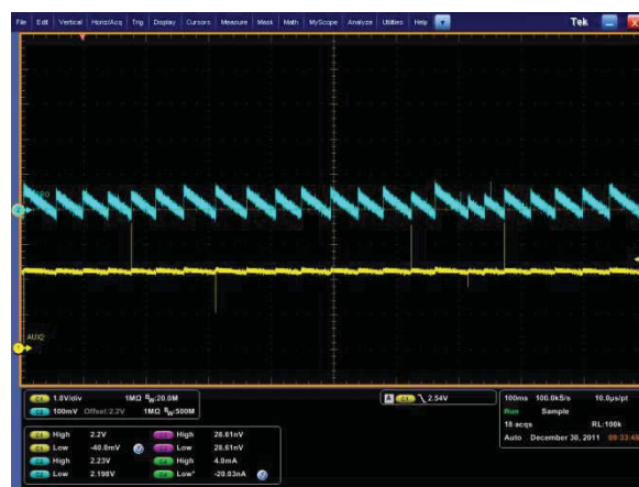
Figure 40. BUCK MINI Output Ripple V IN = 3.6V, V O = 2.5V, I O = 50mA
