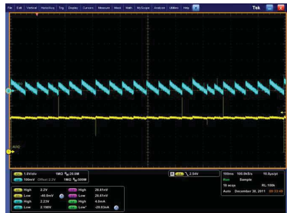
Figure 40. BUCK MINI Output Ripple V IN = 3.6V, V O = 2.5V, I O = 50mA
