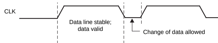
Figure 5-12. Bit Transfer on the Serial Interface
