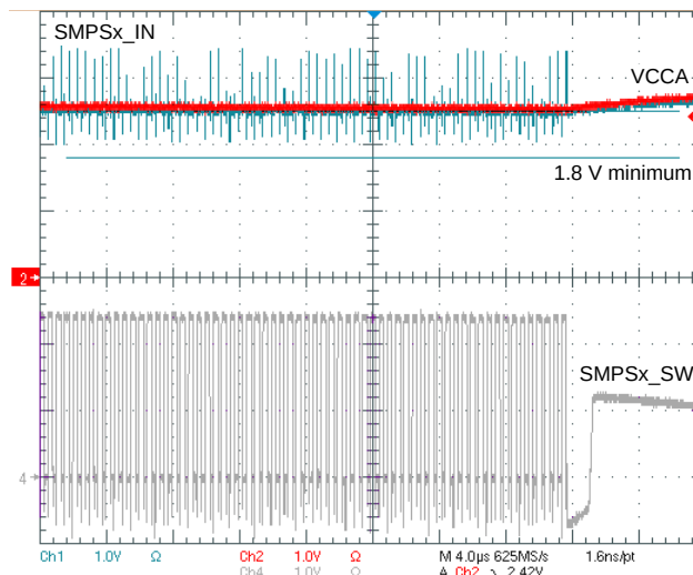
Figure 6-5. Waveform of SMPSx_IN Transients
