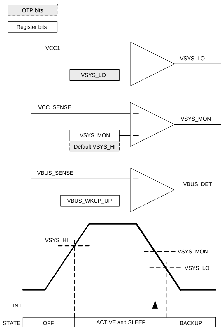
Figure 5-28. System Comparators
