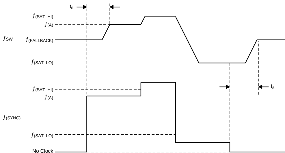
Figure 5-2. Sync Clock Saturation and Frequency Fallback
