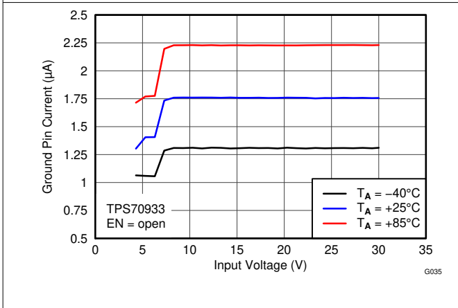
Figure 6-15. GND Current vs V_{IN} and Temperature
