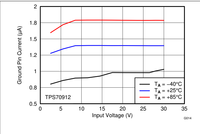
Figure 6-14. GND Current vs V_{IN} and Temperature
