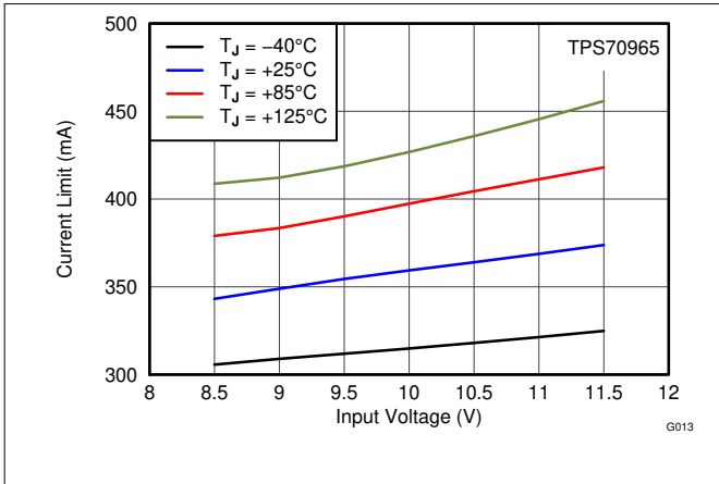
Figure 6-13. 6.5-V Current Limit vs V_{IN} and Temperature
