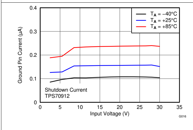
Figure 6-17. Shutdown Current vs V_{IN} and Temperature
