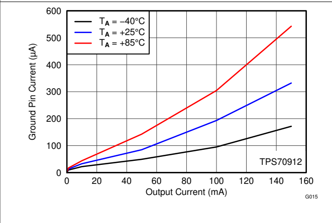
Figure 6-16. GND Current vs I_{OUT} and Temperature
