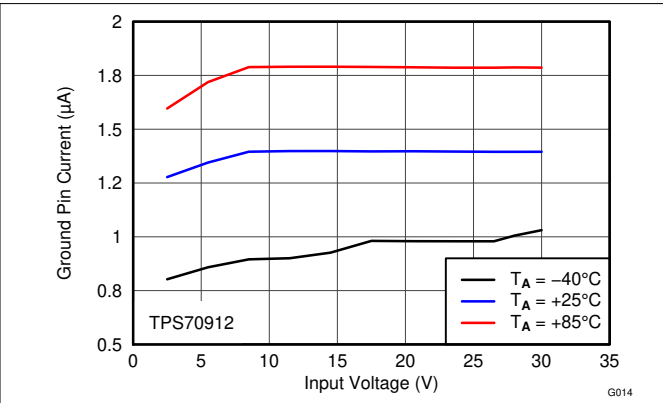
Figure 6-14. GND Current vs V_{IN} and Temperature
