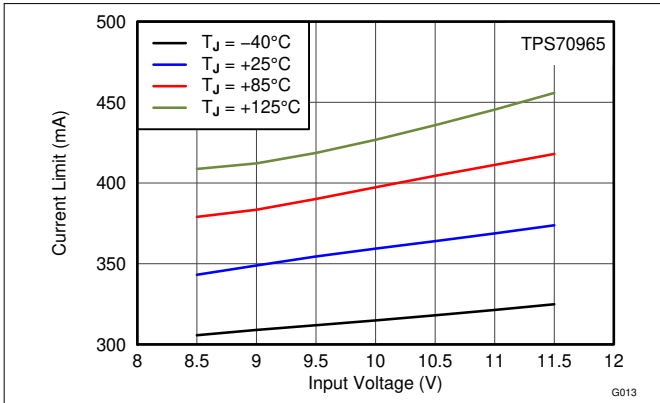
Figure 6-13. 6.5-V Current Limit vs V_{IN} and Temperature
