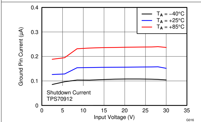
Figure 6-15. GND Current vs V_{IN} and Temperature
