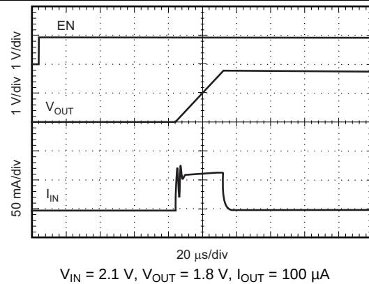
Figure 22. V_{IN} Inrush Current (TPS72718)
