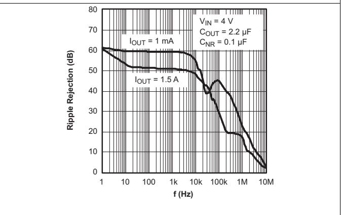
Figure 12. TPS78630 Ripple Rejection vs Frequency
