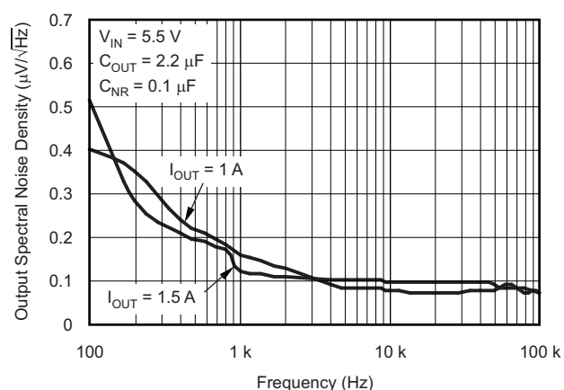
Output Spectral Noise Density vs Frequency TPS79630
