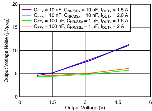
Figure 8. Output Noise vs Output Voltage
