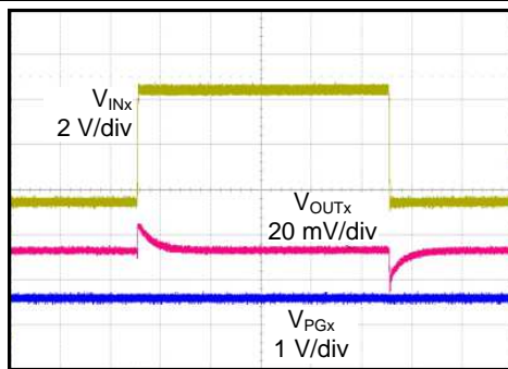
Time (200 \mu\text{s/div} ) V_{\text{IN}x} = 1.4\text{ V to } 6.5\text{ V to } 1.4\text{ V at } 2\text{ V}/\mu\text{s} , V_{\text{OUT}x} = 0.8\text{ V} , I_{\text{OUT}x} = 1\text{ A} , C_{\text{NR/SS}x} = C_{\text{FF}x} = 10\text{ nF}
