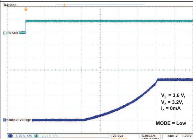
Figure 24. TPS82699 Start-Up
