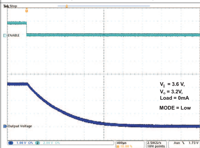
Figure 26. TPS82699 Shutdown
