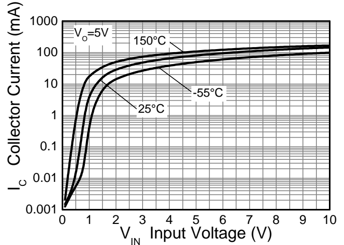
Collector Current v Input Voltage
