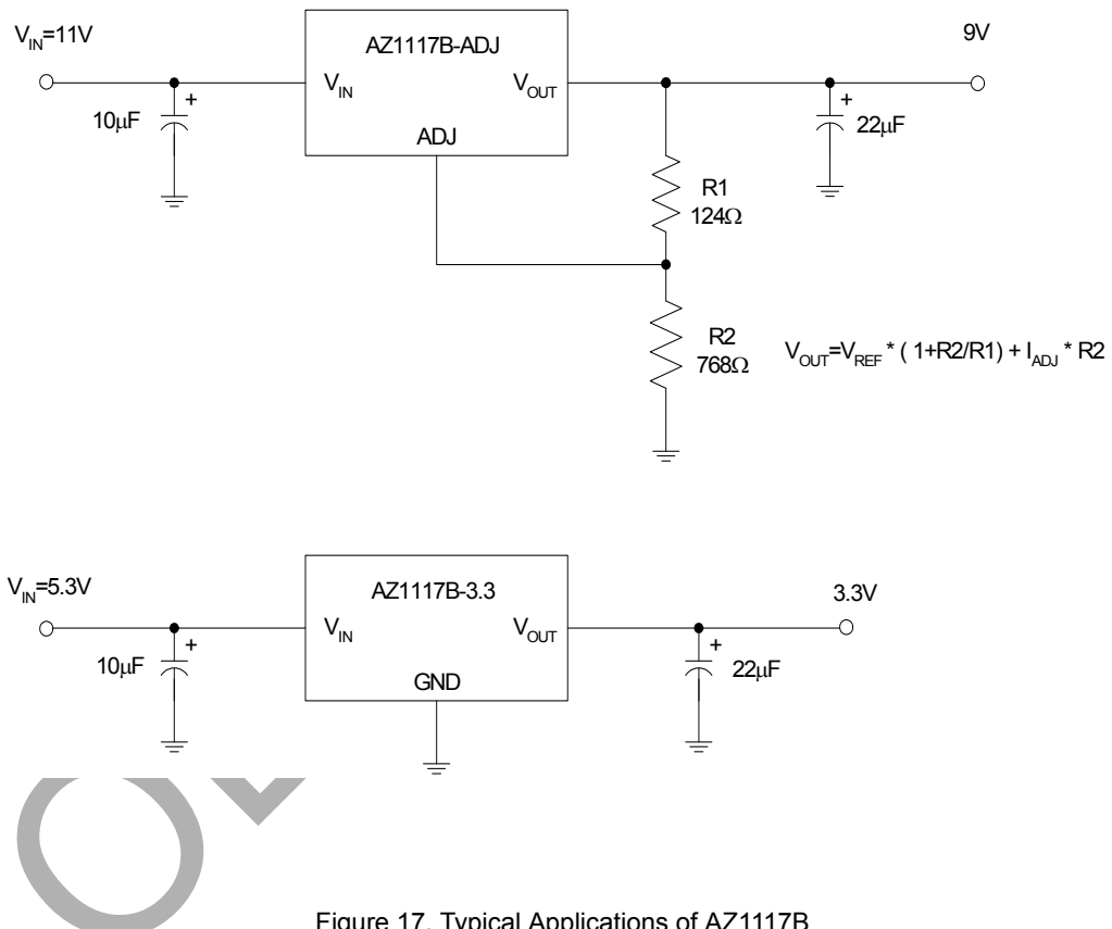
Figure 17. Typical Applications of AZ1117B
