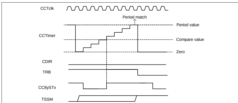
Figure 23-14 Single shot edge aligned - \text{CC8yTC.TSSM} = 1_B , \text{CC8yTC.TCM} = 0_B
