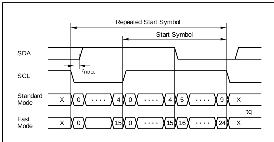
Figure 17-52 Repeated Start Symbol Timing
