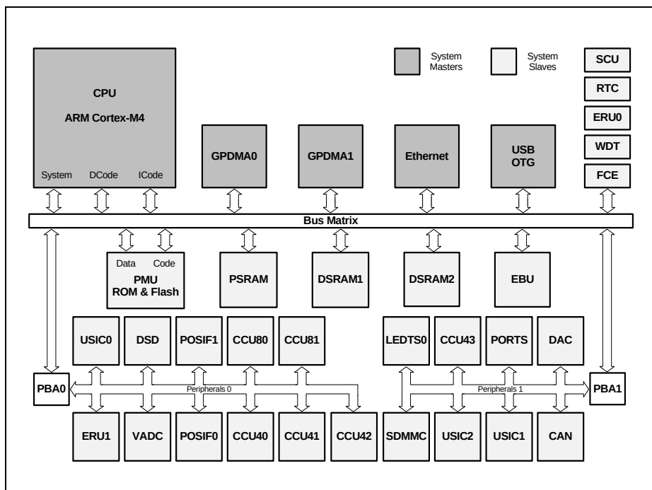
Figure 1-1 XMC4500 System
