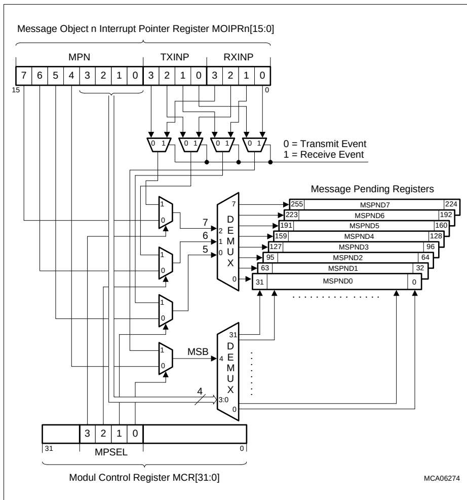
Figure 18-16 Message Pending Bit Allocation
