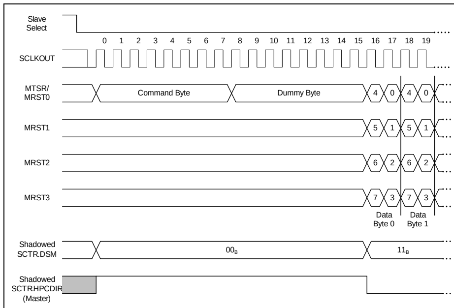
Figure 17-42 Quad-SSC Example
