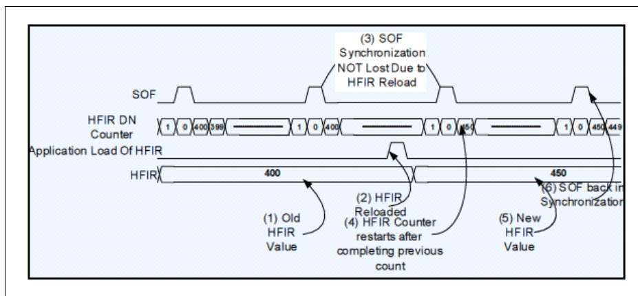
Figure 16-8 Functionality when HFIRIdCtrl = 1 B
