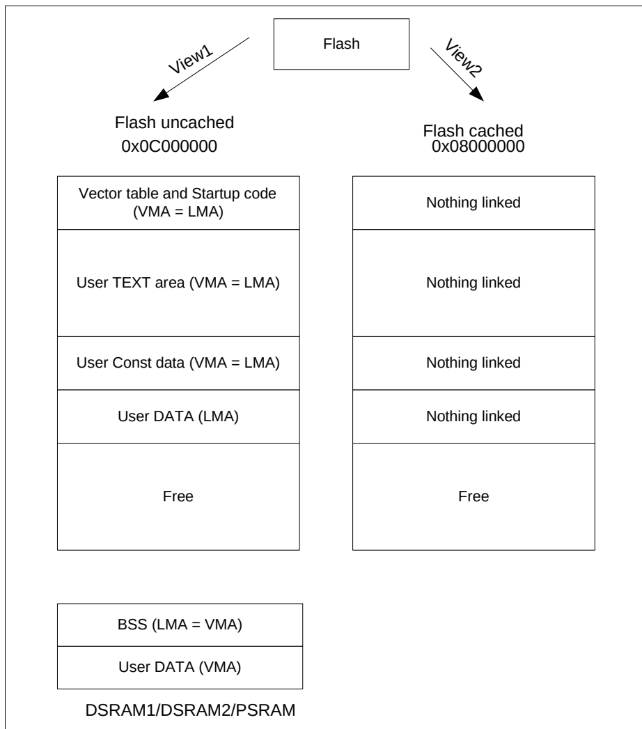
Figure 26-4 Memory Layout1
