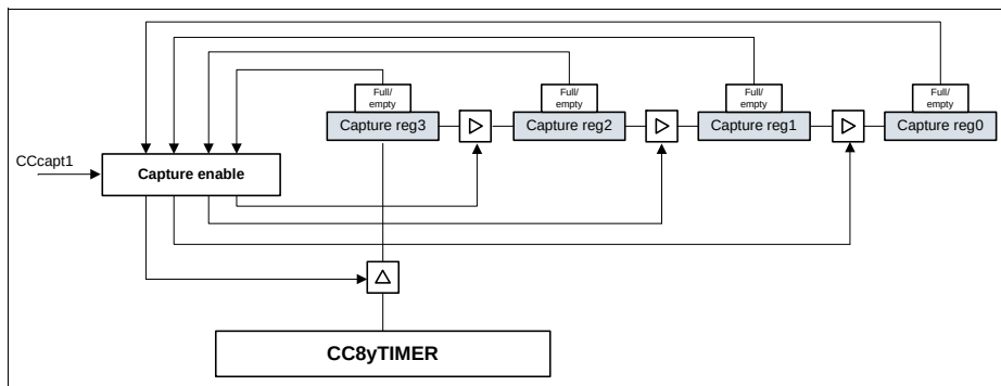
Figure 23-43 Slice Capture Logic - \text{CC8yTC.SCE} = 1_B
