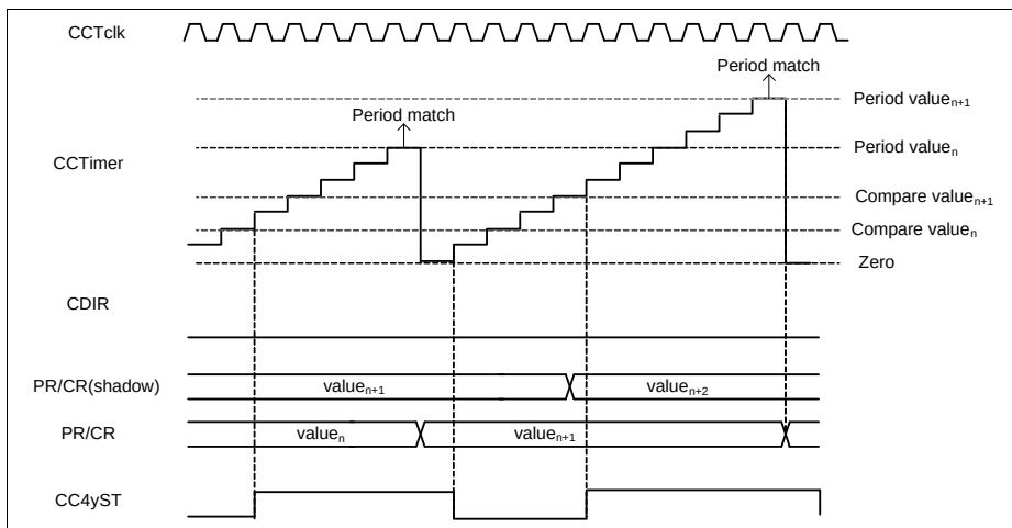
Figure 22-12 Edge aligned mode, \text{CC4yTCM} = 0_B
