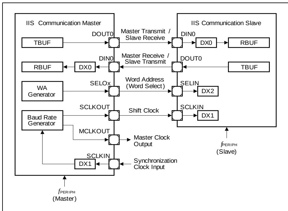
Figure 17-57 IIS Signals
