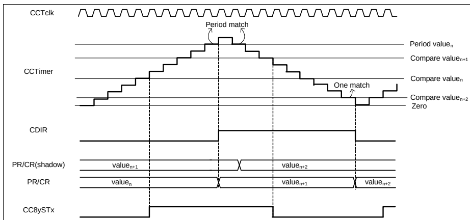
Figure 23-13 Center aligned mode, \text{CC8yTC.TCM} = 1_B
