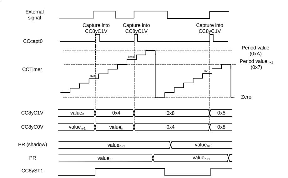
Figure 23-39 External capture - \text{CC8yCMC.CAP0S} \neq 00_B , \text{CC8yCMC.CAP1S} = 00_B
