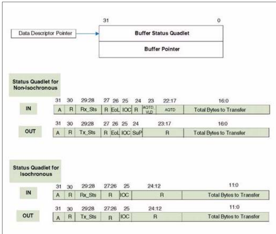
Figure 16-19 Memory Structure
