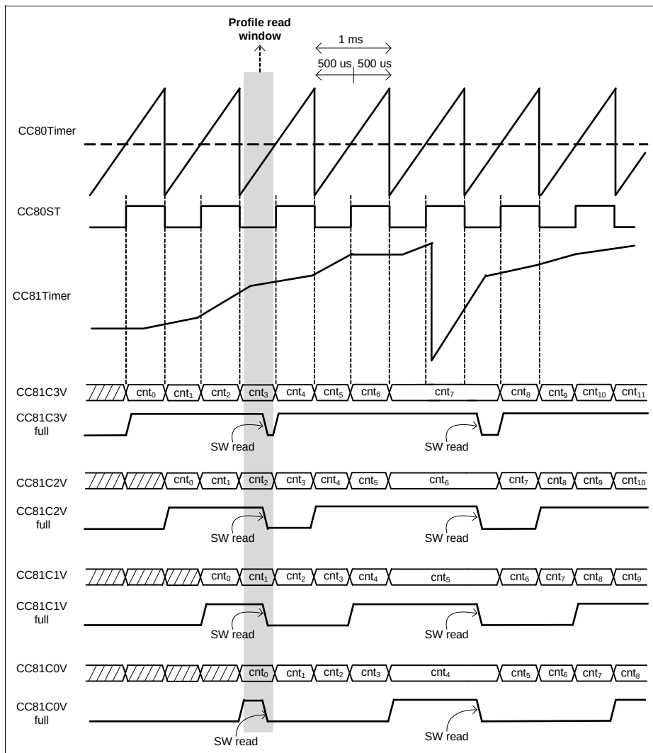
Figure 23-81 Three Capture profiles - CC8yTC.SCE = 1 B
