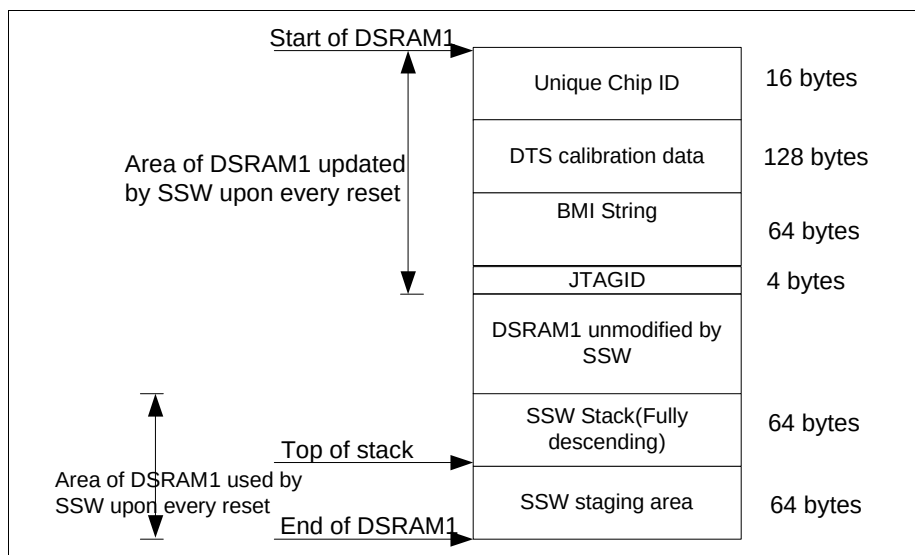
Figure 26-1 DSRAM1 usage by SSW
