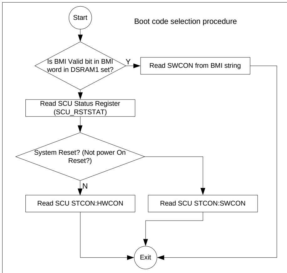
Figure 26-2 Reading Bootcode
