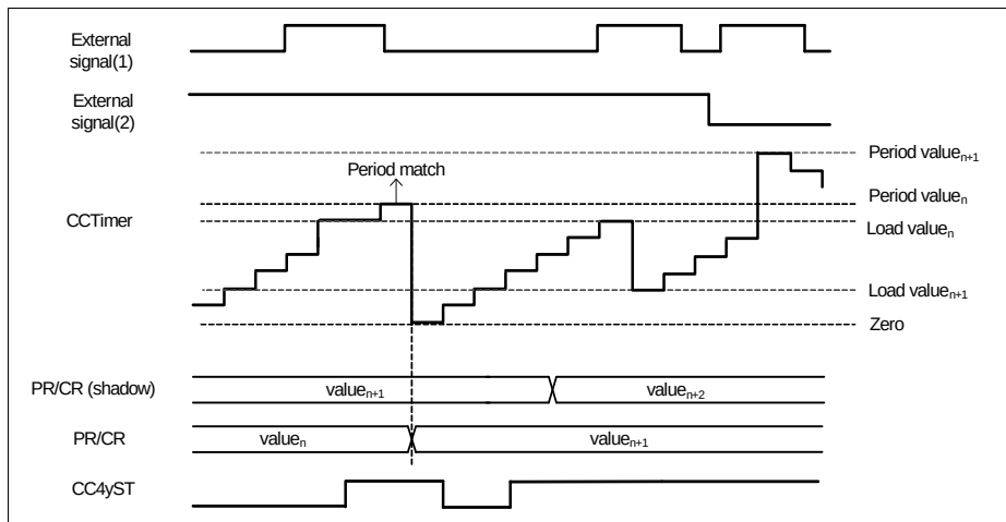
Figure 22-23 External load
