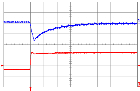
Fig. 1.0V.7: Output voltage response V_{out} = 1.0\text{ V} to positive load current step change from 8 A to 16 A with slew rate of 5 \text{A}/\mu\text{s} at V_{in} = 5\text{ V} . Top trace: output voltage (100 mV/div.); Bottom trace: load current (5 A/div.). C_o = 100\text{ } \mu\text{F} ceramic + 1 \mu\text{F} ceramic. Time scale: 20 \mu\text{s} /div.
