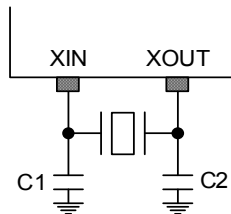
Figure 7.8 Crystal/Ceramic Oscillator
