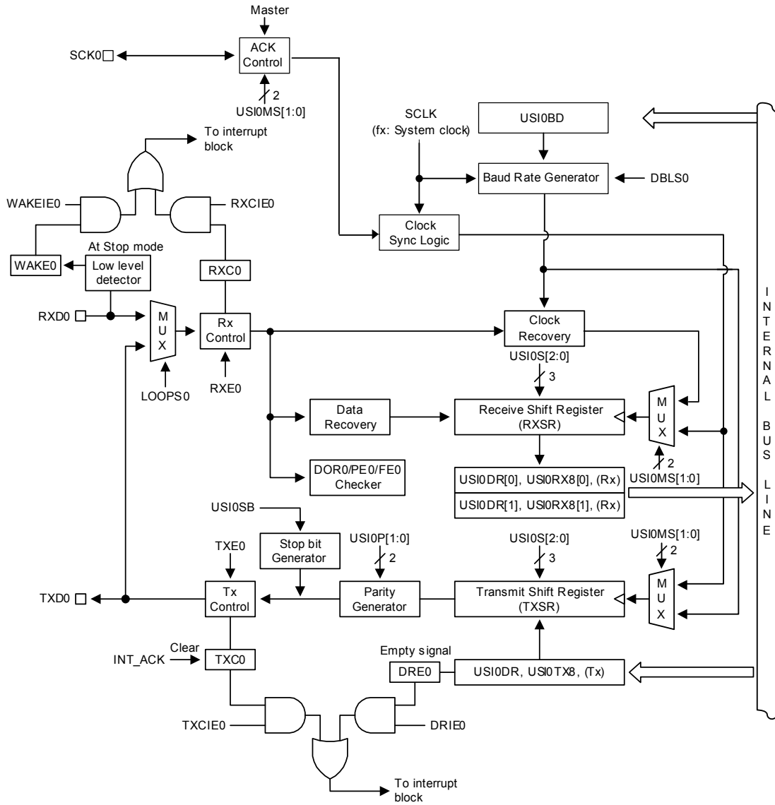
Figure 11.57 USIO UART Block Diagram
