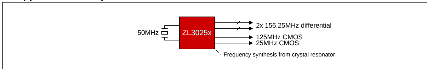
Figure 2 - Ethernet Frequency Synthesis Application
