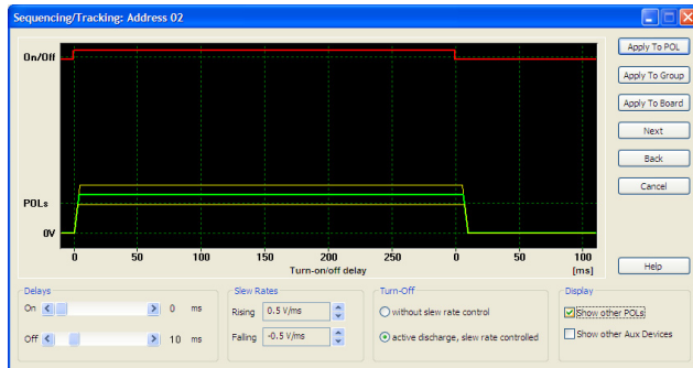
Figure 22. Sequencing/Tracking Window
