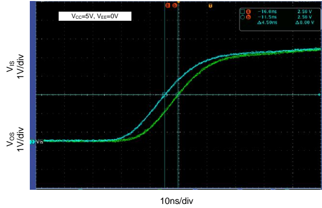
Figure 16. Propagation Delay
