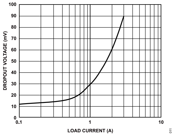
Figure 11. Dropout Voltage ( V_{DROP} ) vs. Load Current ( I_{LOAD} ), V_{OUT} = 1.3 V
