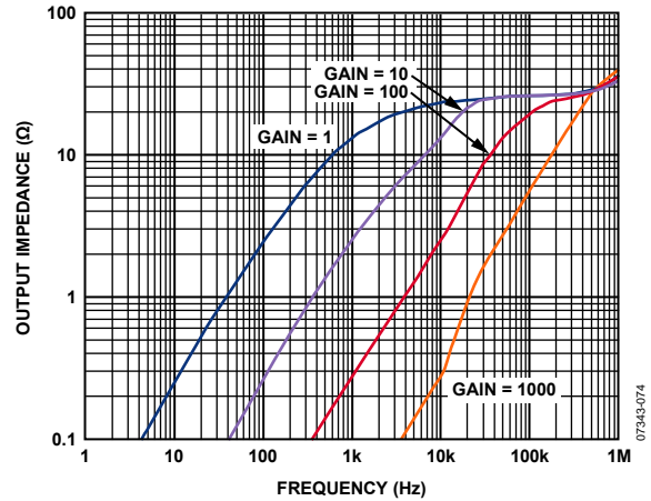
Figure 45. Output Impedance vs. Frequency, G = 1 to 1000
