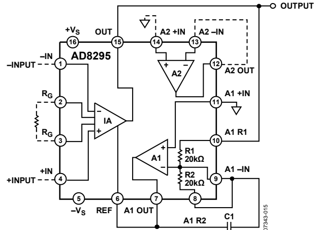
Figure 70. AC-Coupled Connection
