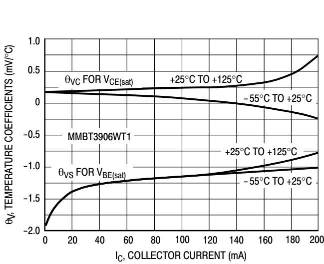
Figure 37. Temperature Coefficients
