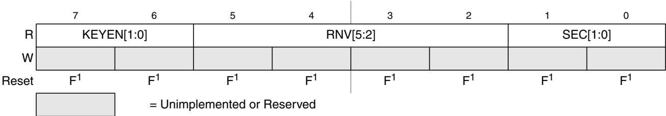
Figure 31-6. Flash Security Register (FSEC)
