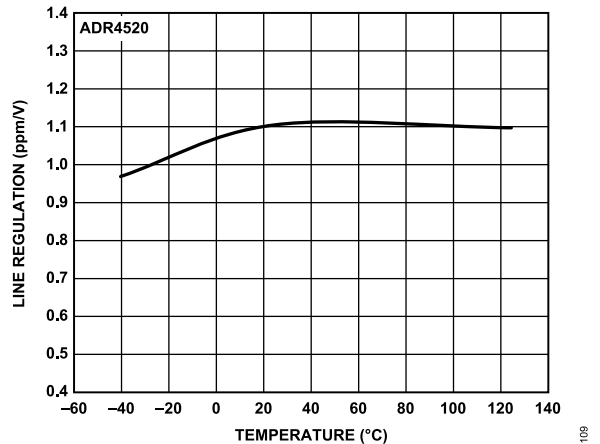
Figure 10. ADR4520 Line Regulation vs. Temperature
