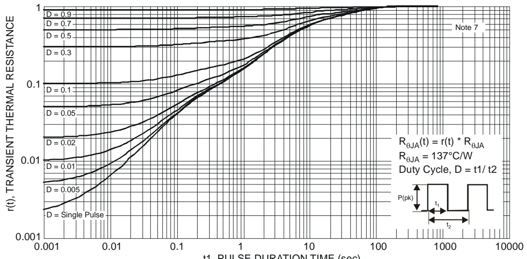
Fig 10 Transient Thermal Resistance B350A-B360A
