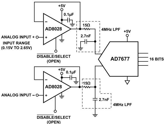
Figure 65. Unity-Gain Differential Drive
