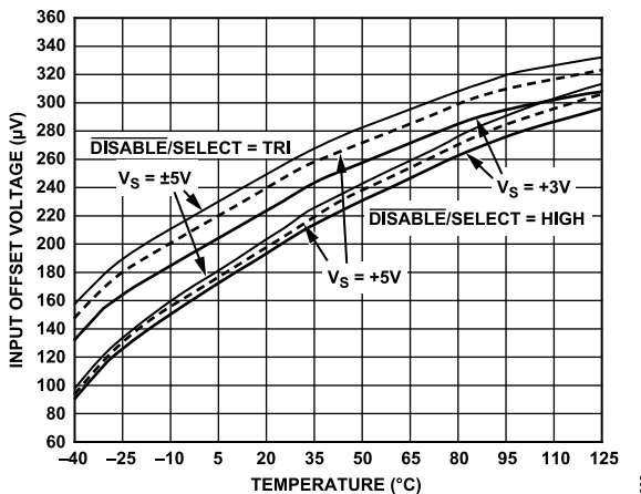
Figure 43. Input Offset Voltage vs. Temperature
