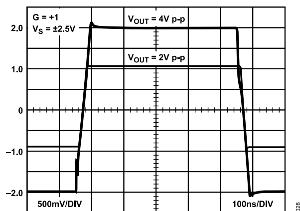
Figure 33. Large Signal Transient Response, G = +1
