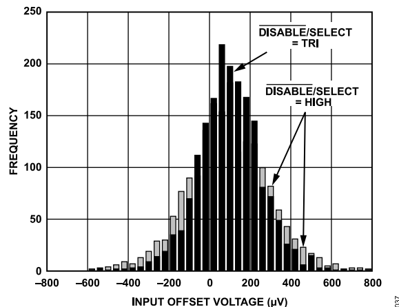
Figure 42. Input Offset Voltage Distribution
