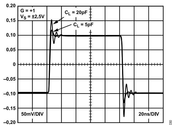
Figure 35. Small Signal Transient Response with Capacitive Load
