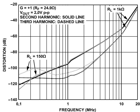
Figure 28. Harmonic Distortion vs. Frequency and Load
