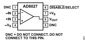
Figure 4. 8-Lead SOIC, AD8027 Pin Configuration
