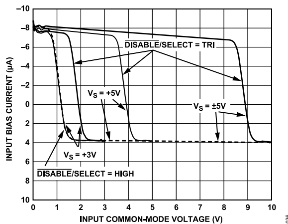
Figure 41. Input Bias Current vs. Input Common-Mode Voltage
