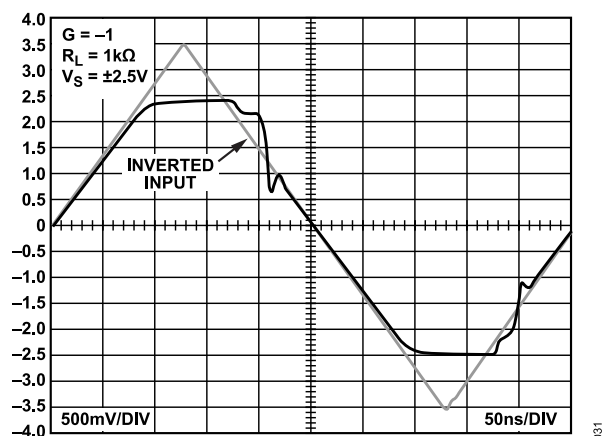
Figure 36. Overdrive Recovery, G = -1
