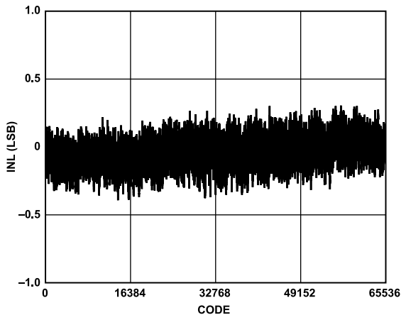
Figure 66. Integral Nonlinearity
