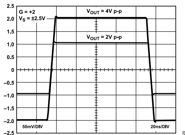
Figure 34. Large Signal Transient Response, G = +2
