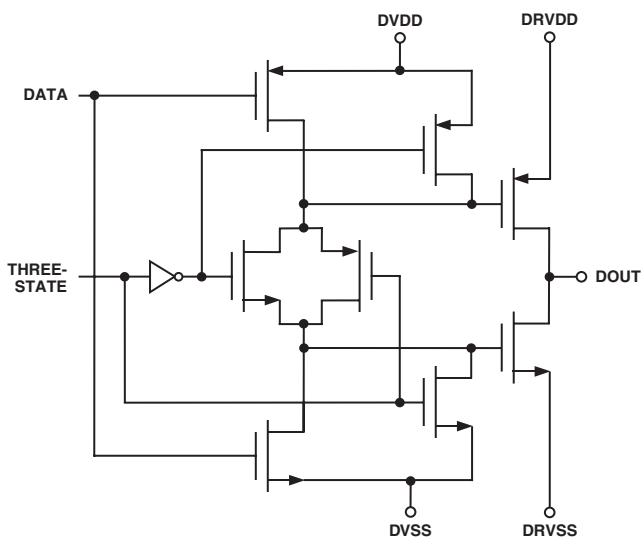
Figure 2. Data Outputs—D0–D11
