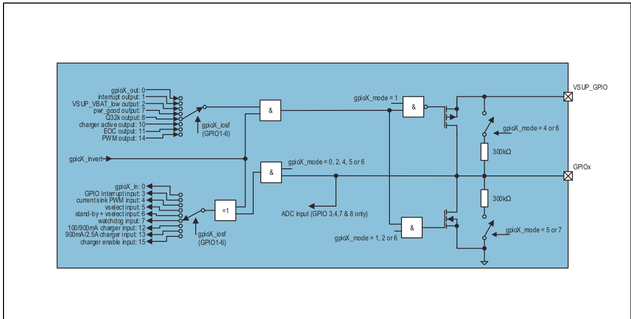
Figure 69: GPIO Block Diagram
