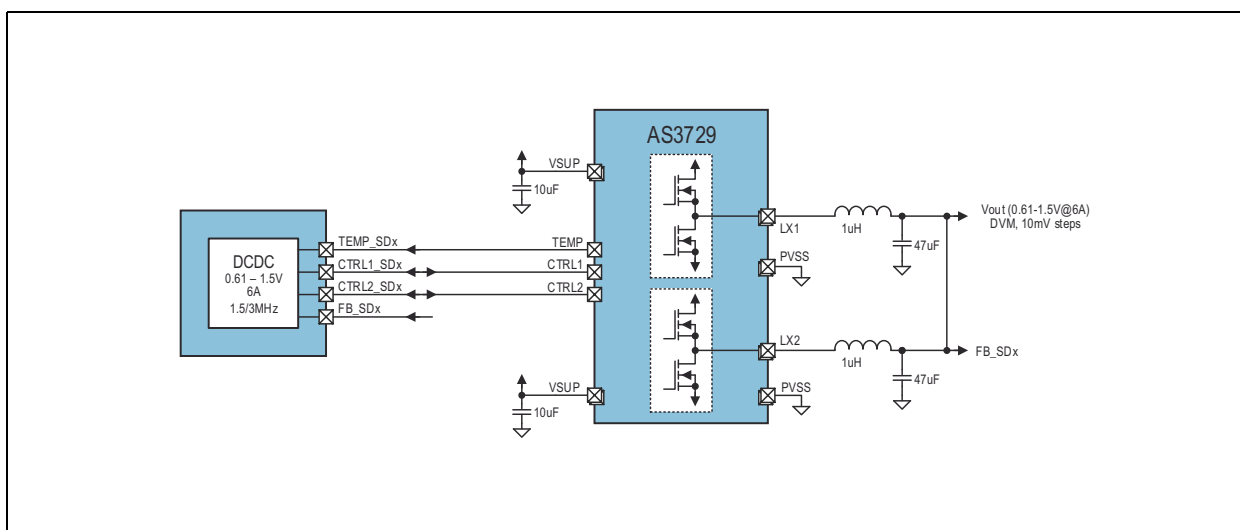
Figure 17: SD4 DC/DC Buck Controller 6A Block Diagram
