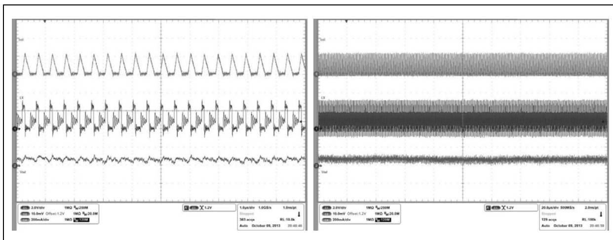
Figure 9: DC/DC Buck Dis-Continuous Mode
