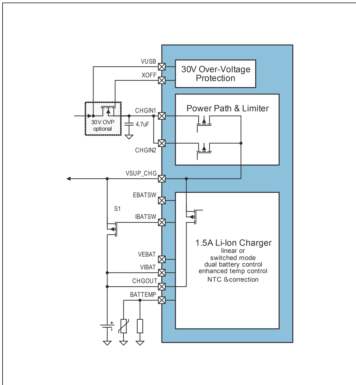
Figure 44: Charger Application Block Diagram, Linear Mode Single Power-Path and Battery
