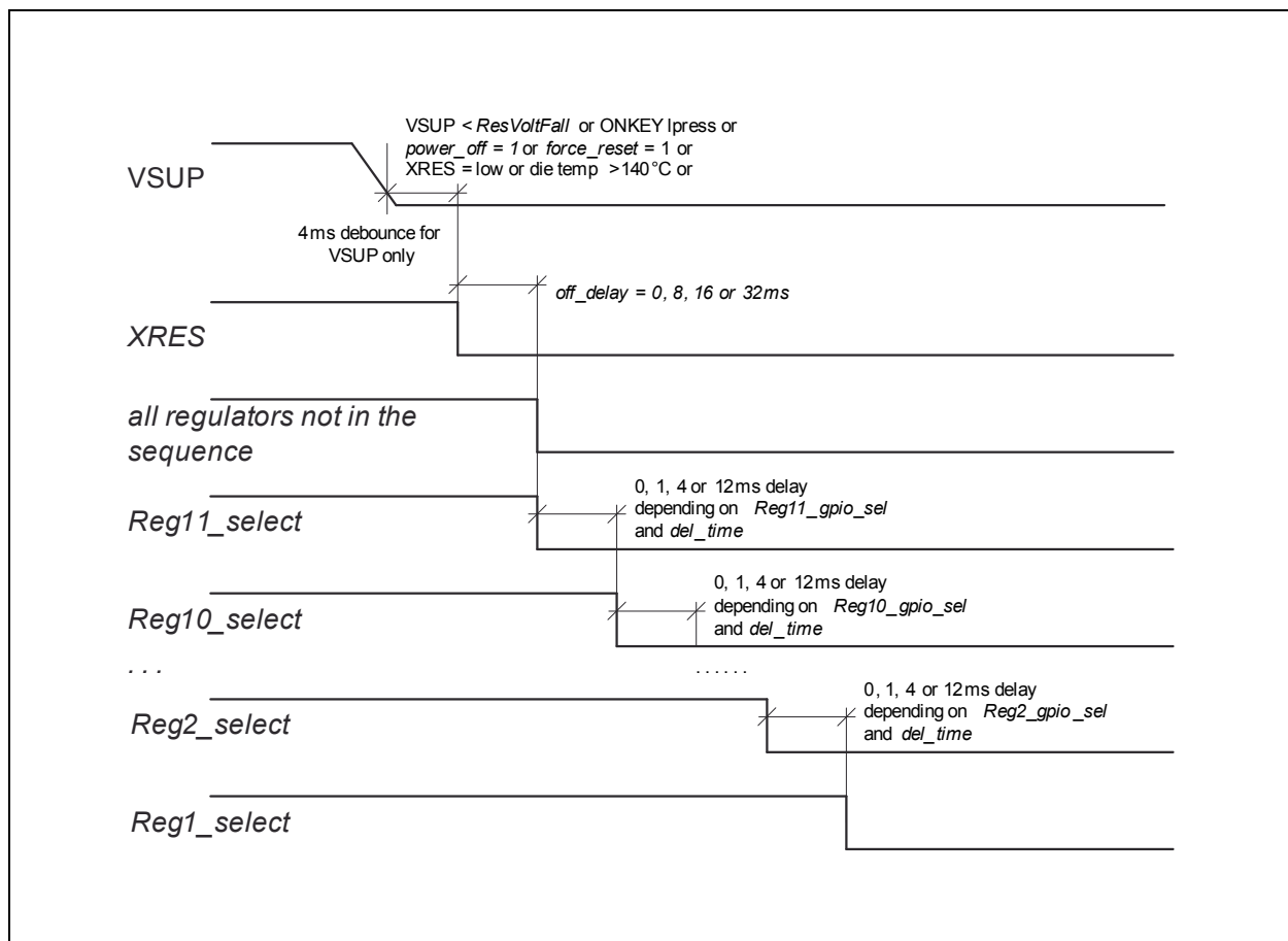
Figure 62: Regulator Power-Down Sequence
