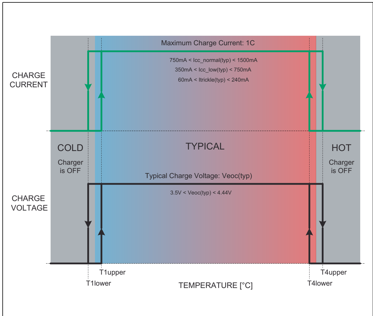
Figure 48: MIN/MAX Temp Supervision
