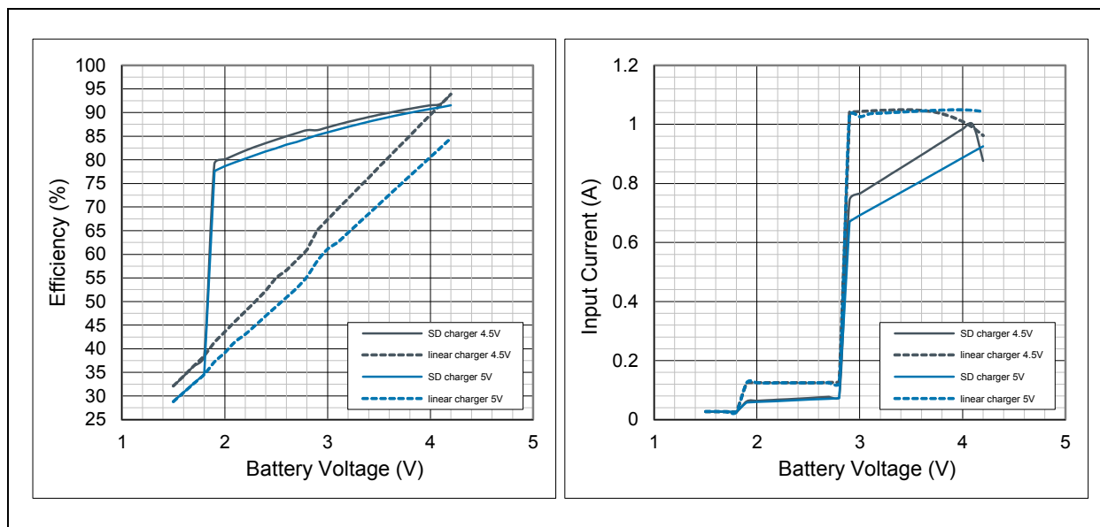
Figure 54: Charger Efficiency and Input Current
