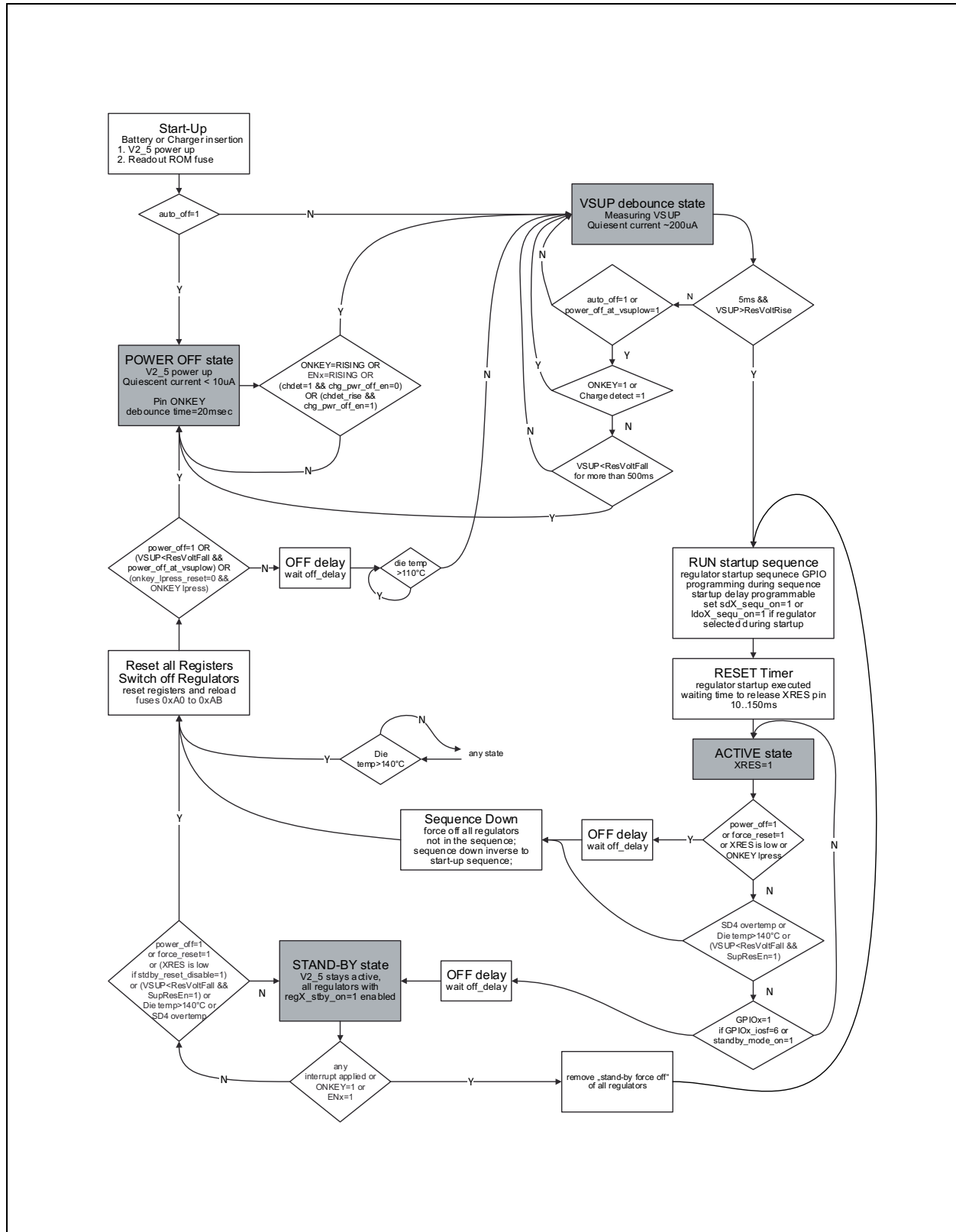
Figure 56: Start-Up Flow Chart
