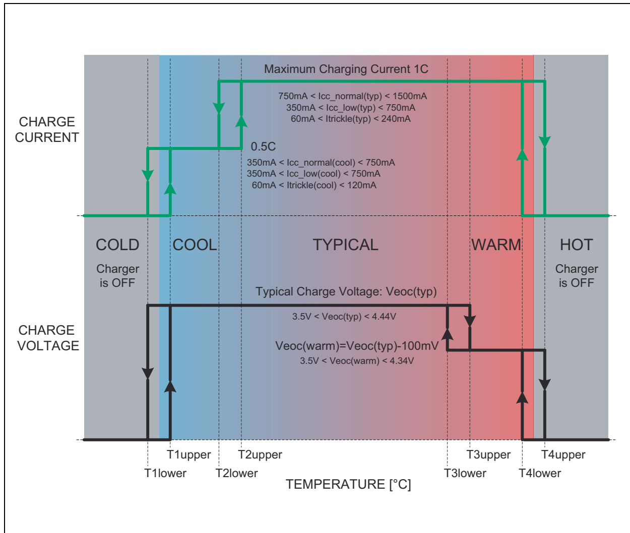
Figure 49: JEITA Temp Supervision
