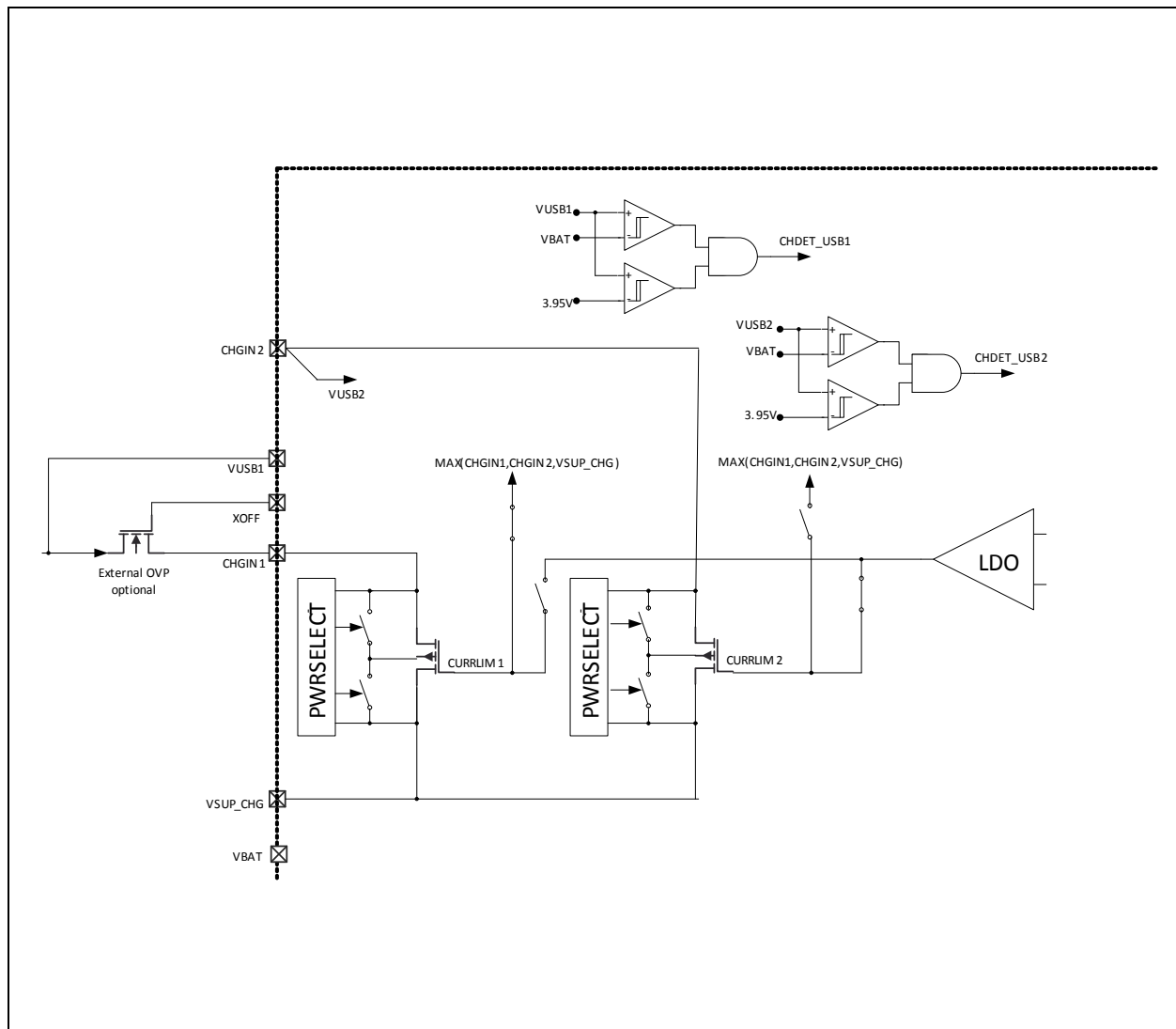
Figure 51: Dual Power Path Diagram
