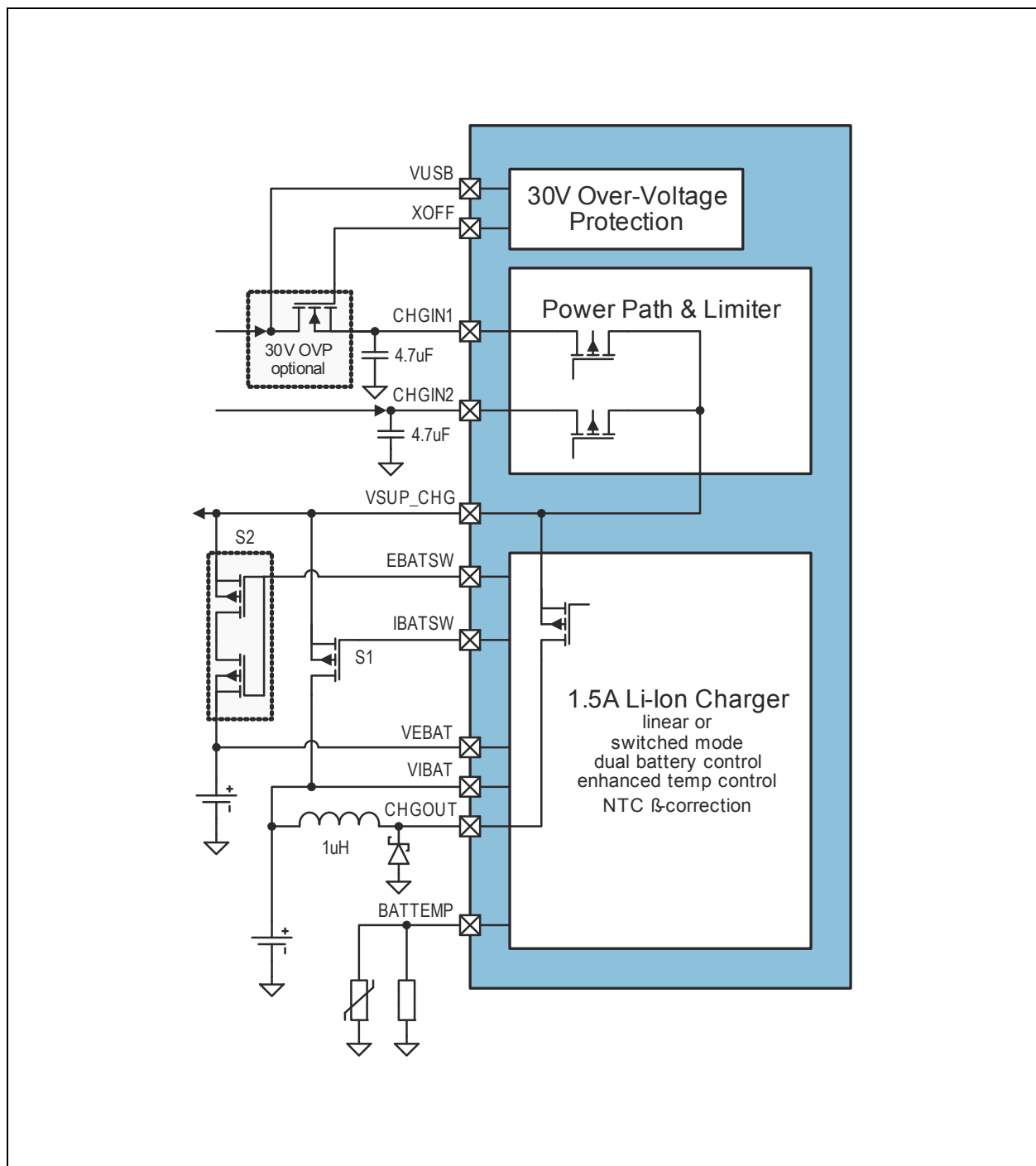
Figure 42: Charger Application Block Diagram, Switch Mode Charger
