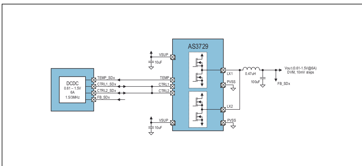
Figure 18: SD4 DC/DC Buck Controller 6A Combined Mode
