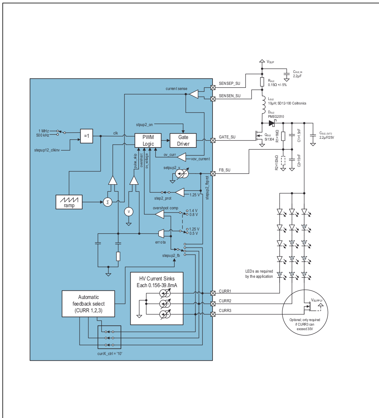
Figure 35: DCDC Step-Up Converter
