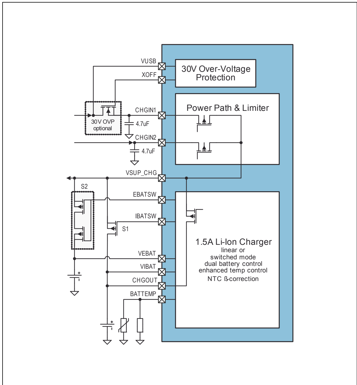
Figure 43: Charger Application Block Diagram, Linear Mode Charger
