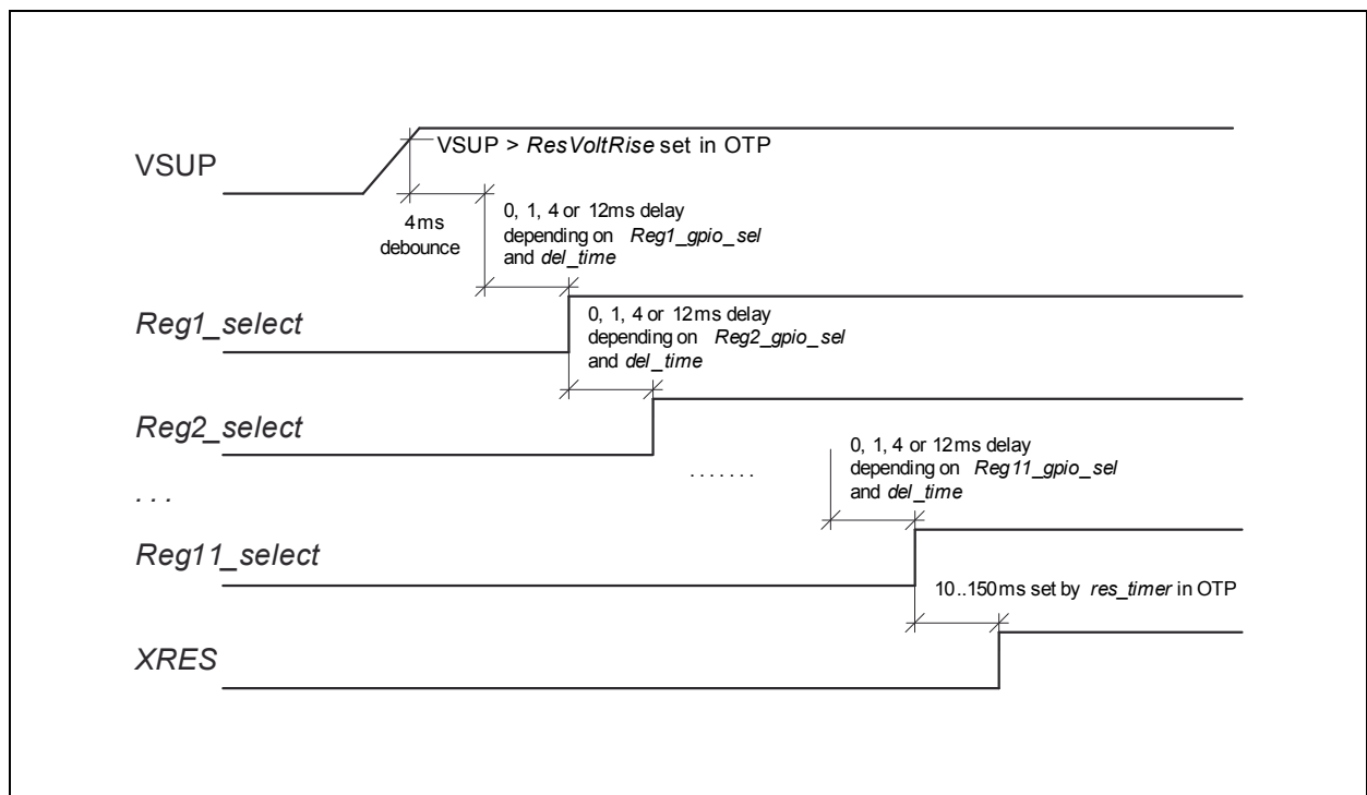
Figure 57: Regulator Power-Up Sequence
