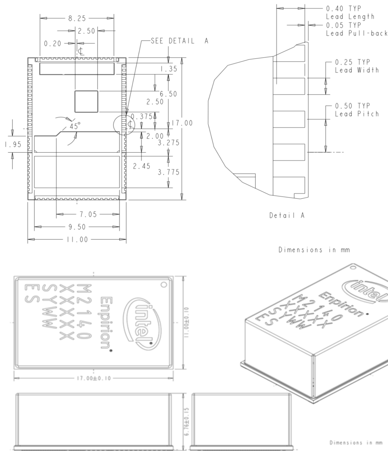
Figure 23: Package Dimensions
