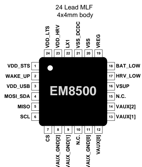
Figure 1-1 QFN24 Package
