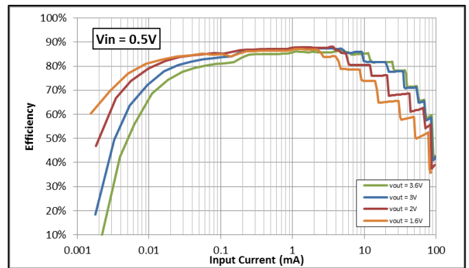
Figure 7-4 Charger Efficiency vs Input Current ( V_{IN} = 0.5V )
