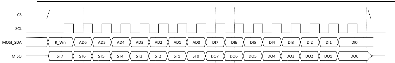
Figure 6-4 SPI transaction scheme CPOL=0, CPHA=0
