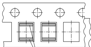
Equivalent terminations because of unipolar component KKE0353-A-E
