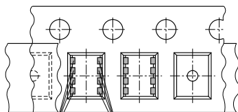
Equivalent terminations because of unipolar component KKE0352-M-E
