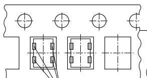
Equivalent terminations because of unipolar component KKE0354-E
