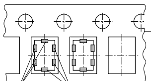
Equivalent terminations because of unipolar component MLV0381-TE
