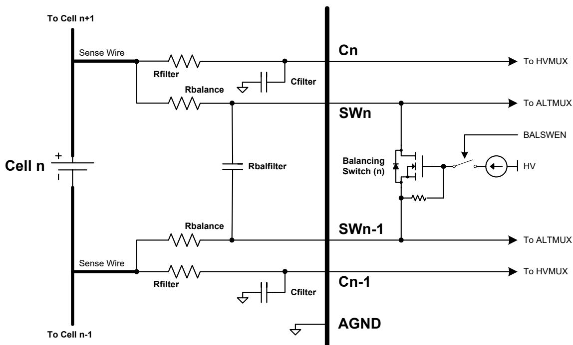
Figure 15. Internal Cell-Balancing
