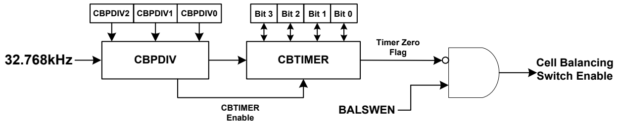
Figure 16. Cell-Balancing Watchdog
