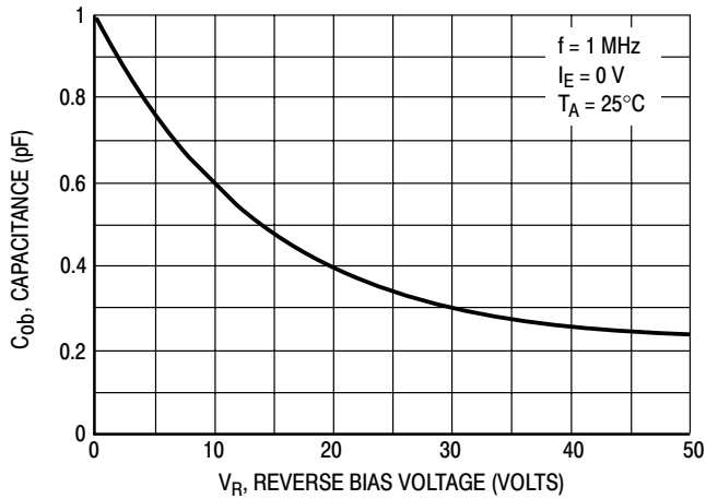
Figure 14. Output Capacitance
