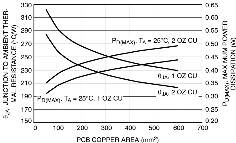
Figure 62. θ JA and P D(MAX) vs. Copper Area (TSOP5)
