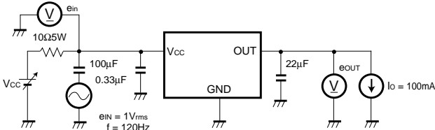
Fig. 2 Measurement circuit for ripple rejection ratio
