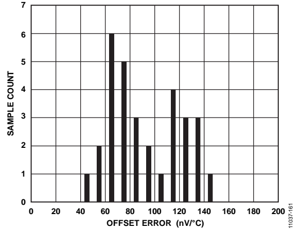
Figure 32. Offset Error Drift Distribution Histogram (Internal Short)
