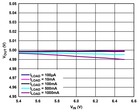
Figure 6. Output Voltage ( V_{OUT} ) vs. Input Voltage ( V_{IN} )
