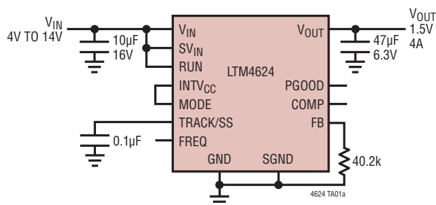
4A, 1.5V Output DC/DC \mu Module Step-Down Regulator
