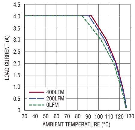
Figure 10. 5V to 1V Derating Curve, No Heat Sink
