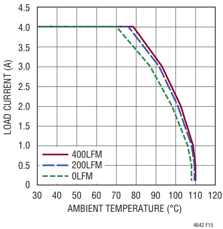
Figure 15. 12V to 3.3V Derating Curve, No Heat Sink
