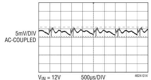
Output Ripple
