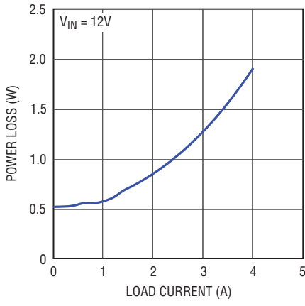
Figure 9. 5V Loss
