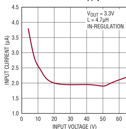
LT8645S No-Load Supply Current
